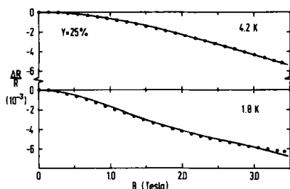
Fig. 1 Negative MR of (\text{CHI}_{0.25})_x at high temperatures. The solid lines are fits of Eq.(1).
